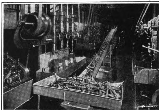
Fig. 16—In the Ford Motor Co.'s plant, application of work-carrying troughs is not limited to the handling of pieces of cylindrical form. Many small parts are carried in this way, but it is necessary to have a considerably greater pitch where the work must slide instead of roll in the trough. This idea is simple and could be used to excellent advantage in handling a great variety of work
